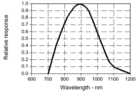
Fig. 5 Spectral Responsivity
