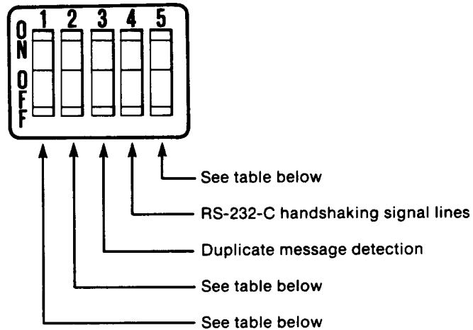
Figure C.2 The Switches on Switch Assembly SW-1
