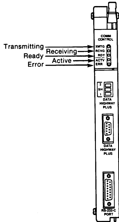
Figure 2.1 1785-KE Communication Interface Module
