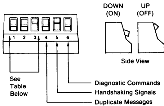
Figure 3.2 The Switches on Switch Assembly SW-1
