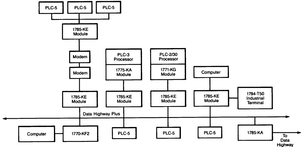
Figure 2.2 A Typical Data Highway Plus Configuration
