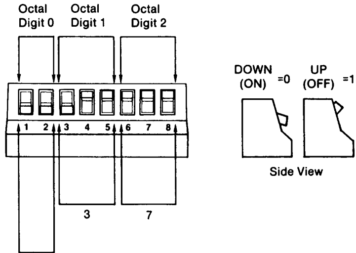
Figure 3.5 Setting the Data Highway Plus Node Address 37
