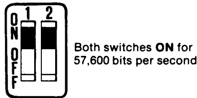
Figure C.5 The Switches on Switch Assembly SW-5
