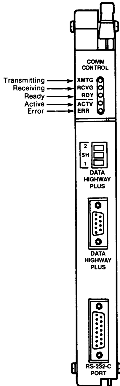
Figure 3.8 The Connectors on the 1785-KE
