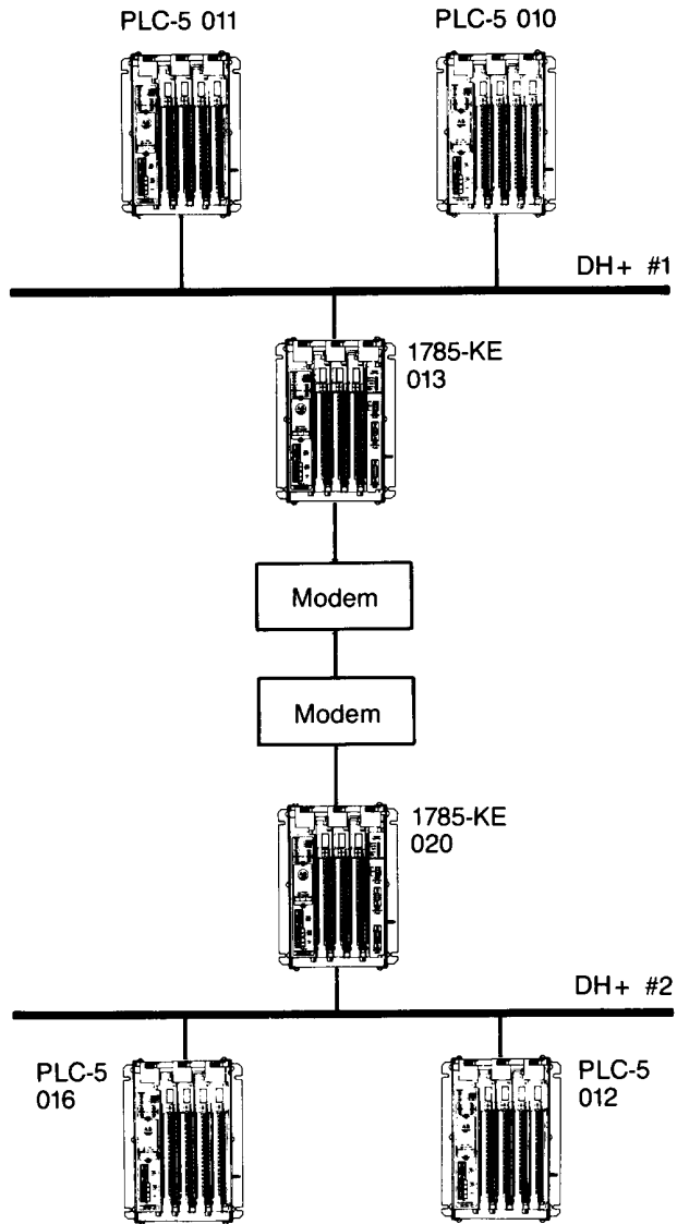
Figure 5.2 Connecting Two Data Highway Plus Networks
