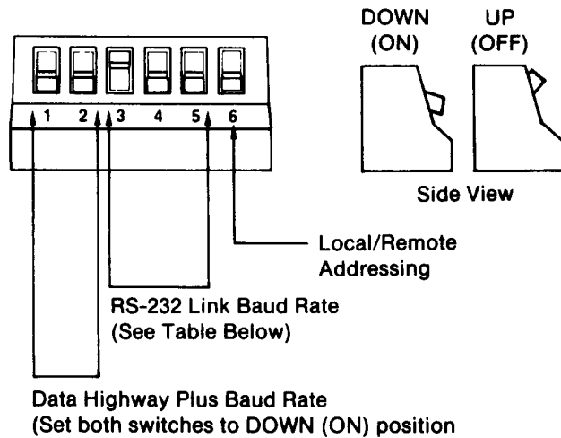
Figure 3.6 Setting Switch Assembly SW-3
