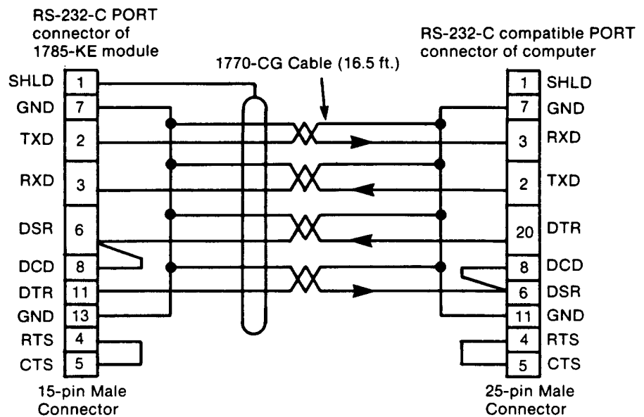
Figure 4.2 Wiring Diagram - RS-232-C PORT Connector to Computer
