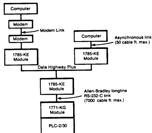
Figure 2.3 Point-to-Links to a Data Highway Plus Network
