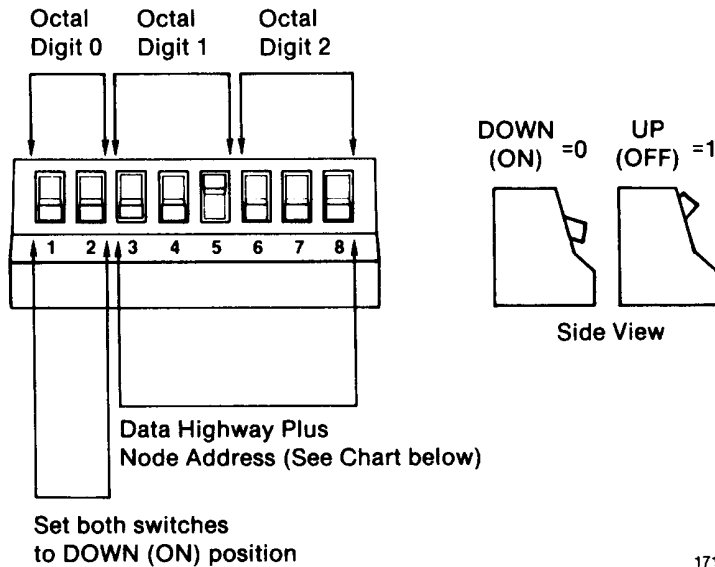
Figure 3.3 Setting Switch Assembly SW-2
