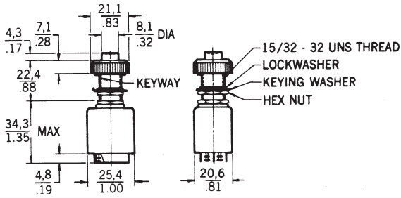
Watertight Switch
