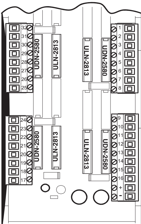
PS-4100-12-P32
