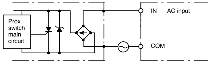
AC Switching
