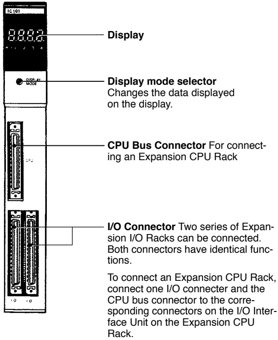
CV500-IC101
