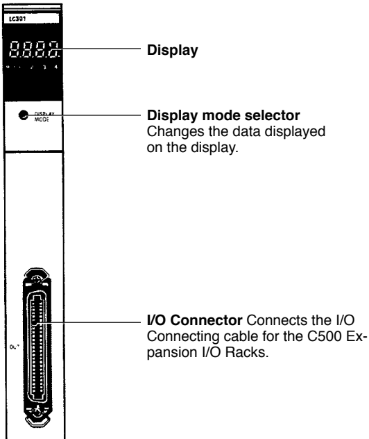
CV500-IC301
