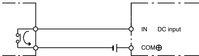
Contact output
