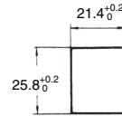
Panel Cutout
