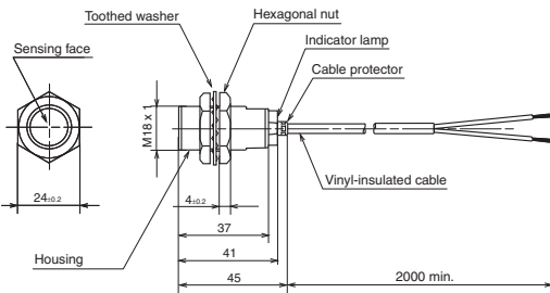
Vinyl-insulated cable (oil-resistant: 0.5mm 2 , 20/0.18, 2-core), dia. 5.7. Cap color: blue.
