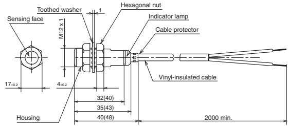
Numbers in parentheses indicate dimensions for the G type. Vinyl-insulated cable (oil-resistant: 0.3mm 2 , 27/0.12, 2-core), dia. 4.1. Cap color: blue.
