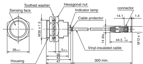
Vinyl-insulated cable (vibration- and oil-resistant): 0.5mm 2 , 20/0.18, 2-core), dia. 5.7. Cap color: blue.
