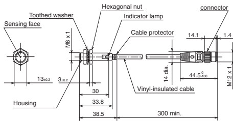
Vinyl-insulated cable (vibration- and oil-resistant): 0.3mm 2 , 27/0.12, 2-core), dia. 4.1. Cap color: blue.
