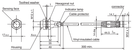
Vinyl-insulated cable (vibration- and oil-resistant): 0.3mm 2 , 27/0.12, 2-core), dia. 4.1. Cap color: blue.
