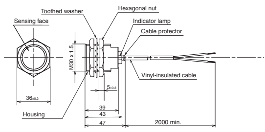
Vinyl-insulated cable (oil-resistant: 0.5mm 2 , 20/0.18, 2-core), dia. 5.7. Cap color: blue.
