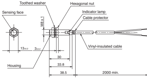
Vinyl-insulated cable (oil-resistant: 0.3mm 2 , 27/0.12, 2-core), dia. 4.1. Cap color: blue.
