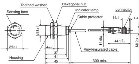
Vinyl-insulated cable (vibration- and oil-resistant): 0.5mm 2 , 20/0.18, 2-core), dia. 5.7. Cap color: blue.
