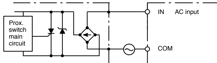
AC Switching
