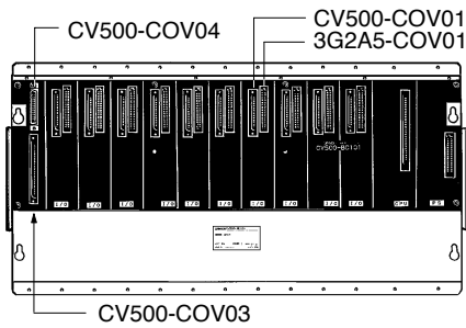
CPU Rack
