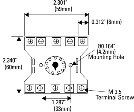
SR3P-06 Socket
