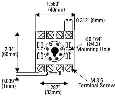
SR2P-06 Socket
