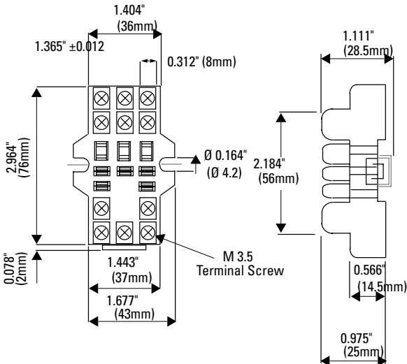
SR3B-05 Socket
