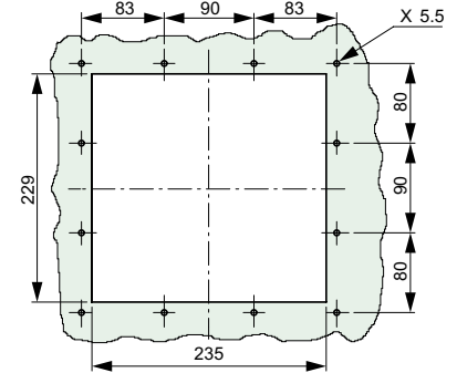
Mounting opening
