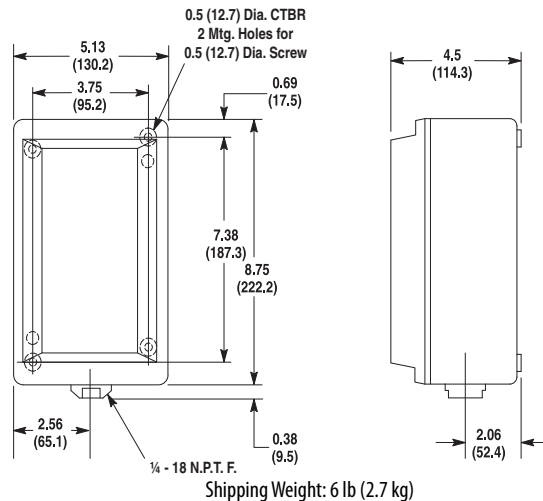
Figure 27 - Type 4X
