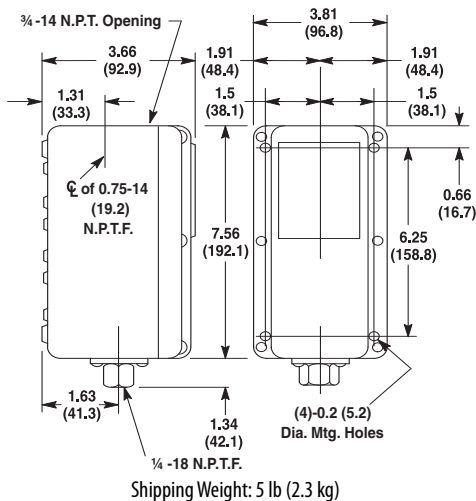
Figure 26 - Type 4 & 13
