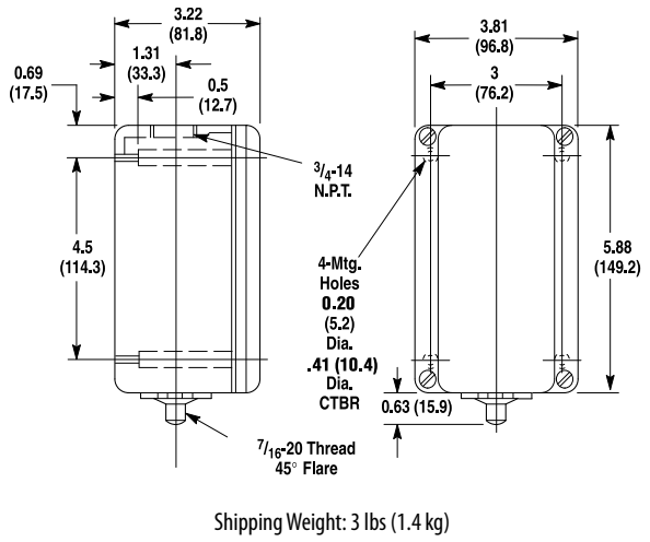
Figure 19 - Type 4 & 13
