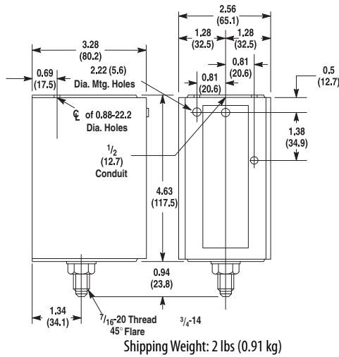
Figure 18 - Type 1
