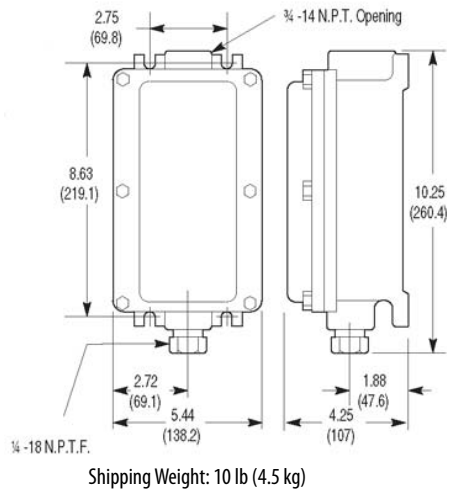
Figure 27 - Type 4X
