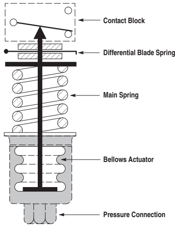
Figure 3 - Basic Mechanical Structure
