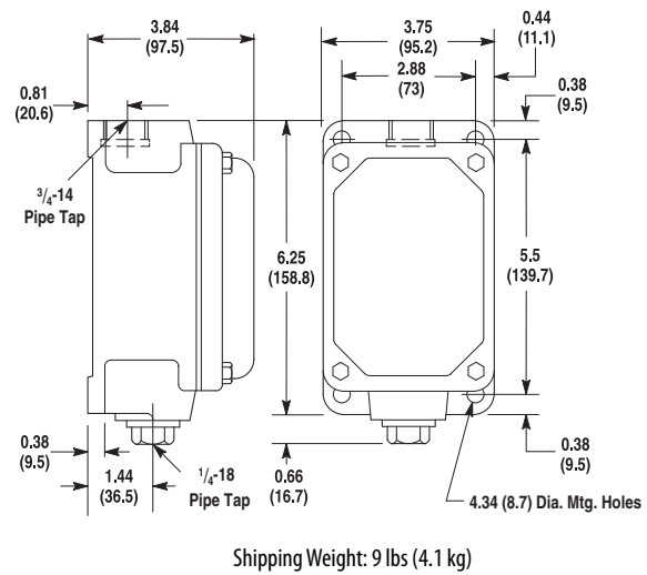
Figure 20 - Type 7 & 9 and 4 & 13
