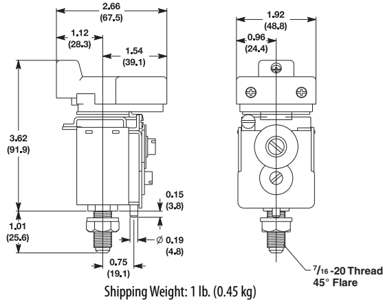
Figure 17 - Open Type
