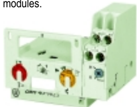
Trip module ZMR-...-PKZ 2 1) plugs into the PKZ 2 Disconnect to complete starter. Includes 1N.O. & 1 N.C overload relay trip & signalling contacts. See page 7/26 for more info on ZMR-...-PKZ 2 trip modules.
