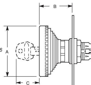
2-Position Trigger Action Mushroom and Mushroom Key Release Operator 60 mm
