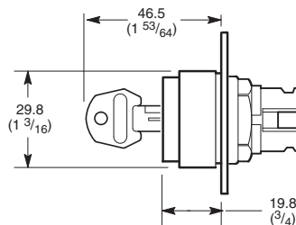
Low Profile Key Selector Switch Operators
