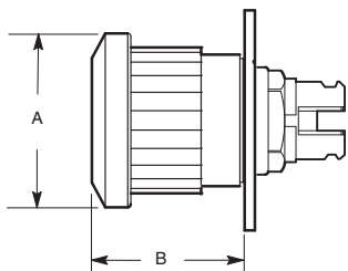
2-Position Push-Pull Mushroom Operators Illuminated and Non-Illuminated 40 mm and 60 mm
