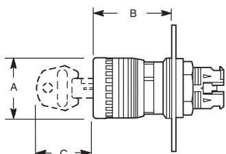
2-Position Trigger Action Twist-to-Release Operator 30 mm and Mushroom Key Release Operator 30 mm
