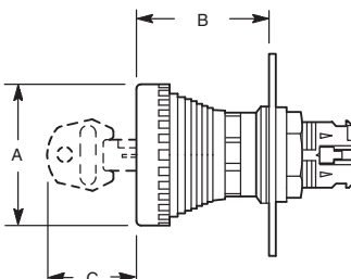
2-Position Trigger Action Mushroom and Mushroom Key Release Operator 40 mm
