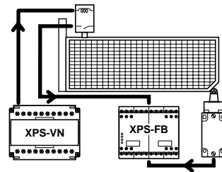
Interlocking Device with Electromagnetic Lock
