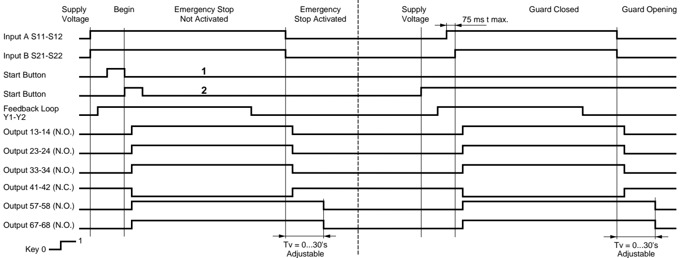
Functional Diagram for XPS-AT Module with Emergency Stop Monitoring
