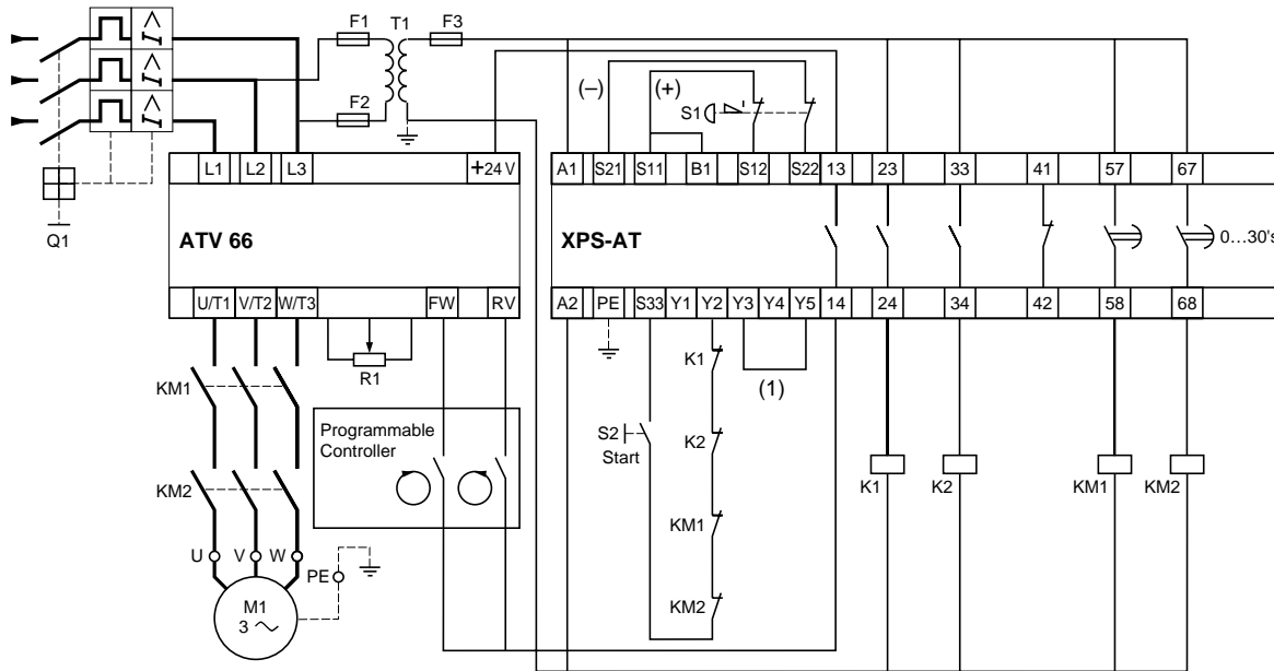
(1) With start button monitoring S1: Emergency stop button with 2 N.C. contacts (recommended application)
