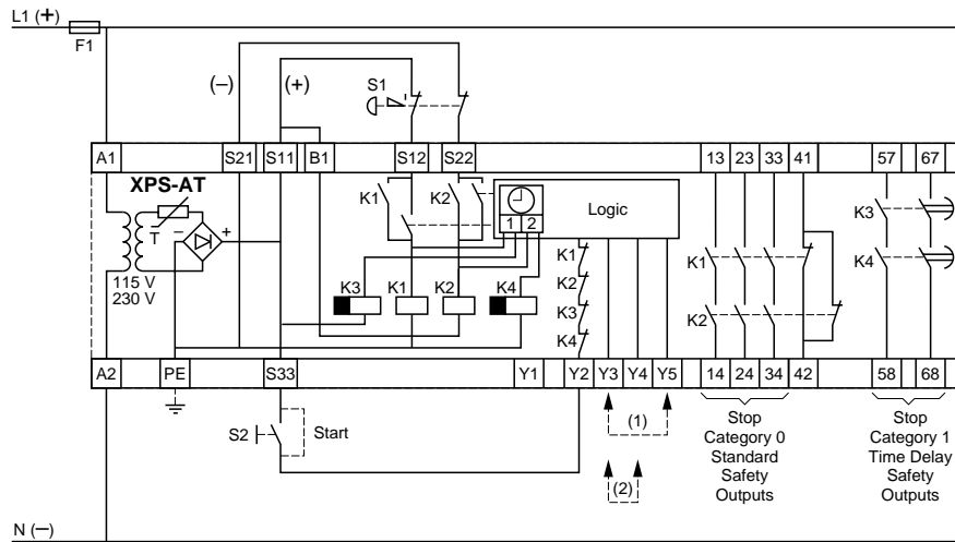
Functional Diagram for XPS-AT Module with Emergency Stop Monitoring
