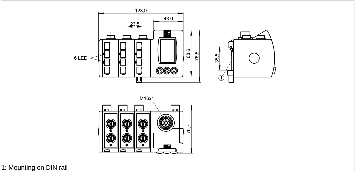
1: Mounting on DIN rail
