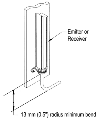
Figure 4. Cable Clearances
