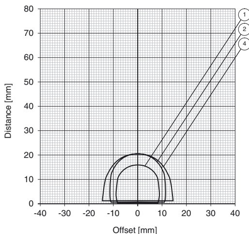
Writing range mounted flush in aluminium IPC03-30GK
