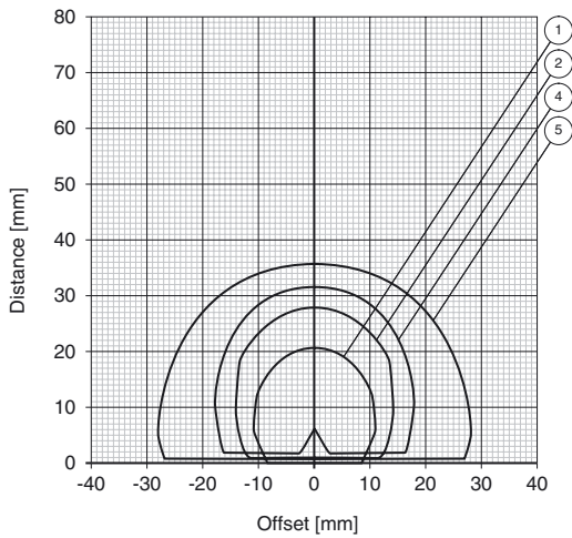
Writing range in air IPC03-30GK
