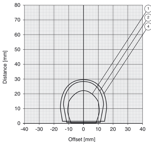
Reading range mounted flush in steel IPC03-30GK
