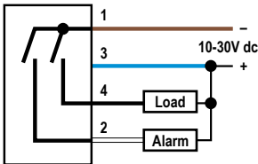
NPN (Sinking) Alarm Wiring
