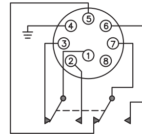
8 PIN SUBSEA CONNECTOR – 8DD SPDT FORM C
