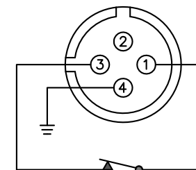
4 PIN MICRO CONNECTOR — DBD SPST FORM B
