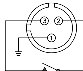
3 PIN MICRO CONNECTOR — DBA SPST FORM A
