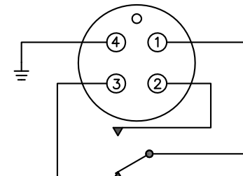
4 PIN SUBSEA CONNECTOR — 4DD SPDT FORM C
