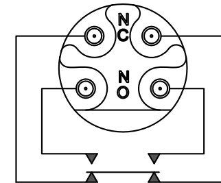
10/20 SERIES TERMINAL DMDB FORM Z
