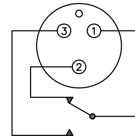
3 PIN SUBSEA CONNECTOR – 3DD SPDT FORM C
